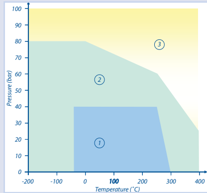
Pressure/Temperature Graph:
