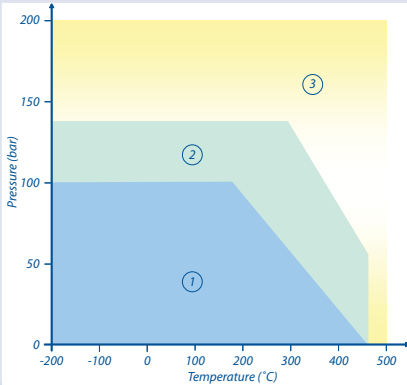
Pressure/Temperature Graph:
