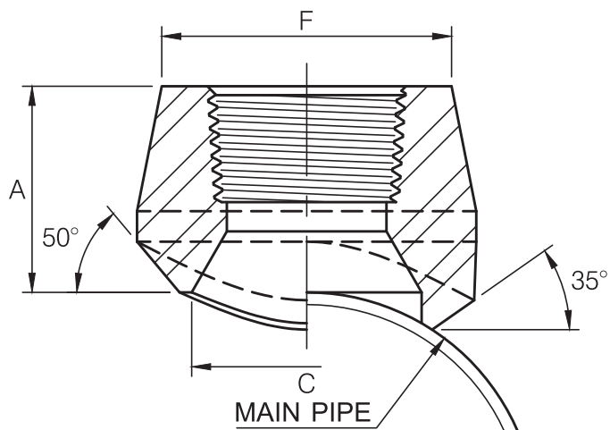
REDUCING WAY
