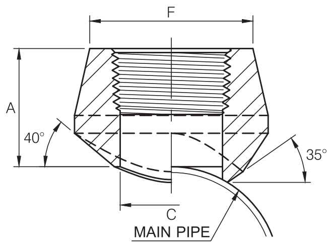
STRAIGHT WAY
