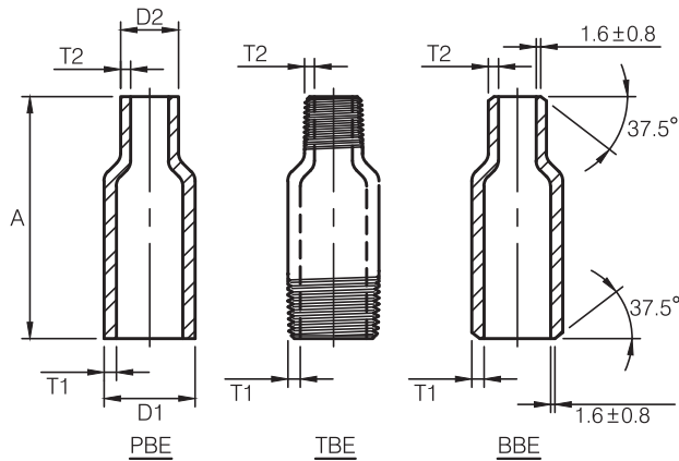
CONCENTRIC
