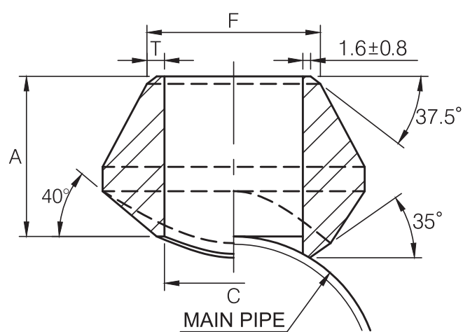
STRAIGHT WAY
