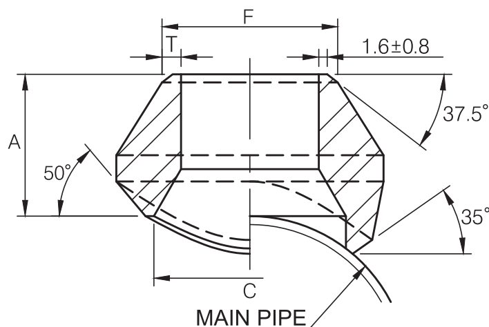
REDUCING WAY
