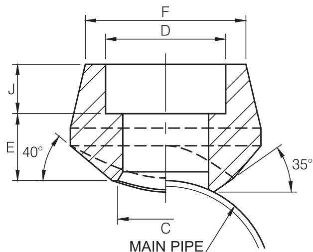
STRAIGHT WAY
