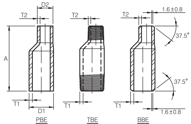
ECCENTRIC
